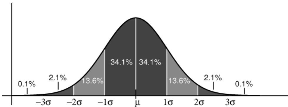
Fig. 13: Normal Distribution
